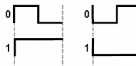
FM0 Symbols
